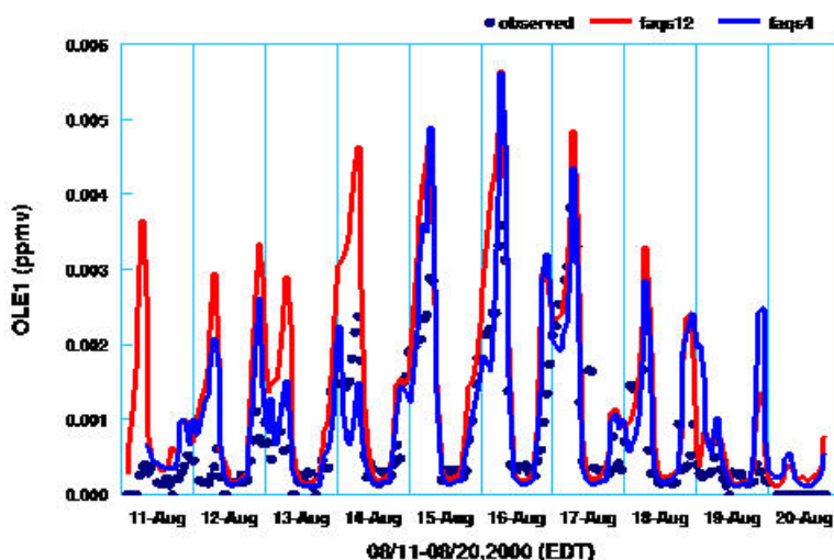
4 5 6 Figure 0.6 Time Series Plot of Simulated and Observed Surface OLE1 Concentrations at PAMS Station with AIRS code of 130890002 in Atlanta
