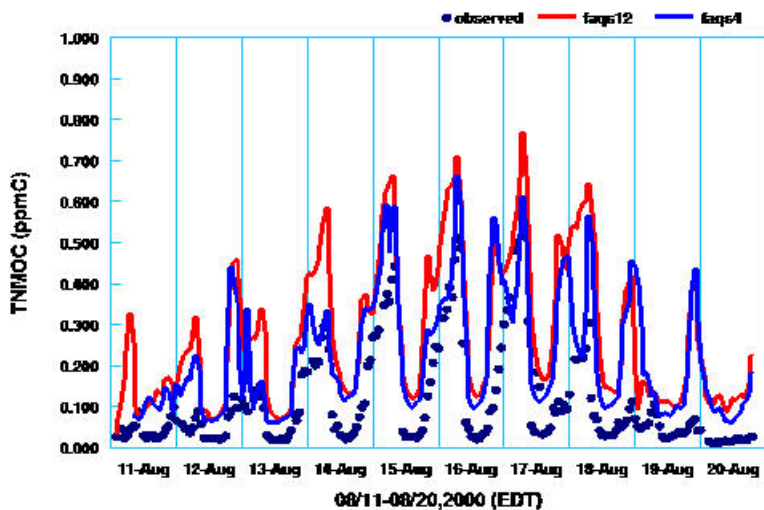
17 18 Figure 0.2 Time Series Plot of Simulated and Observed Surface Total Nonmethan Organic Compounds Concentrations at 19 PAMS Station with AIRS code of 130890002 in Atlanta
