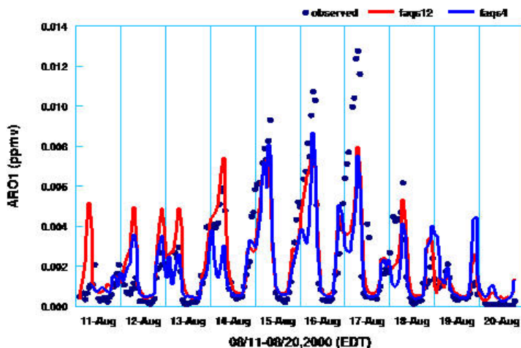
1 2 3 Figure 0.5 Time Series Plot of Simulated and Observed Surface ARO1 Concentrations at PAMS Station with AIRS code of 130890002 in Atlanta
