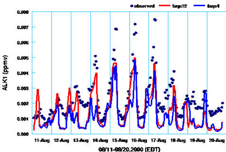
4 5 6 Figure 0.4 Time Series Plot of Simulated and Observed Surface ALK1 Concentrations at PAMS Station with AIRS code of 130890002 in Atlanta
