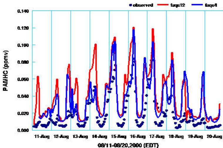
1 2 3 Figure 0.3 Time Series Plot of Simulated and Observed Surface PAMS Hydrocarbons Concentrations at PAMS Station with AIRS code of 130890002 in Atlanta
