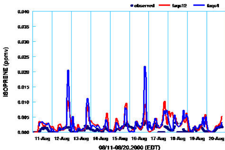
1 2 3 Figure 0.7 Time Series Plot of Simulated and Observed Surface ISOPRENE Concentrations at PAMS Station with AIRS code of 130890002 in Atlanta
