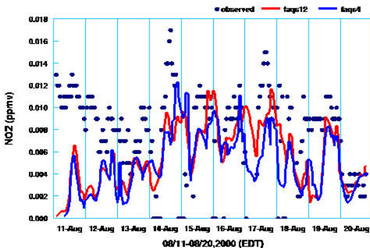
14 15 Figure 0.1 Time Series Plot of Simulated and Observed Surface NOZ Concentrations at PAMS Station with AIRS code of 16 130890002 in Atlanta
