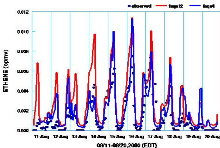
4 5 6 Figure 0.8 Time Series Plot of Simulated and Observed Surface ETHENE Concentrations at PAMS Station with AIRS code of 130890002 in Atlanta
