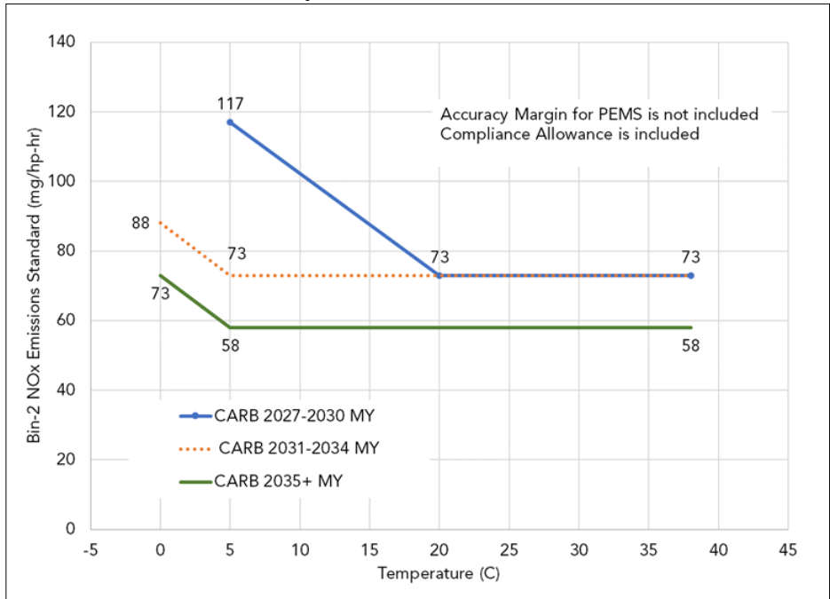
Fig. 1 – CARB Proposal for MHDD & HHDD 1 Bin-2 Off-Cycle NOx Emissions Standards
