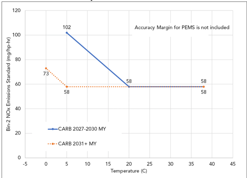
Fig. 2 – CARB Proposal for LHDD 1 Bin-2 Off-Cycle NOx Emissions Standards
