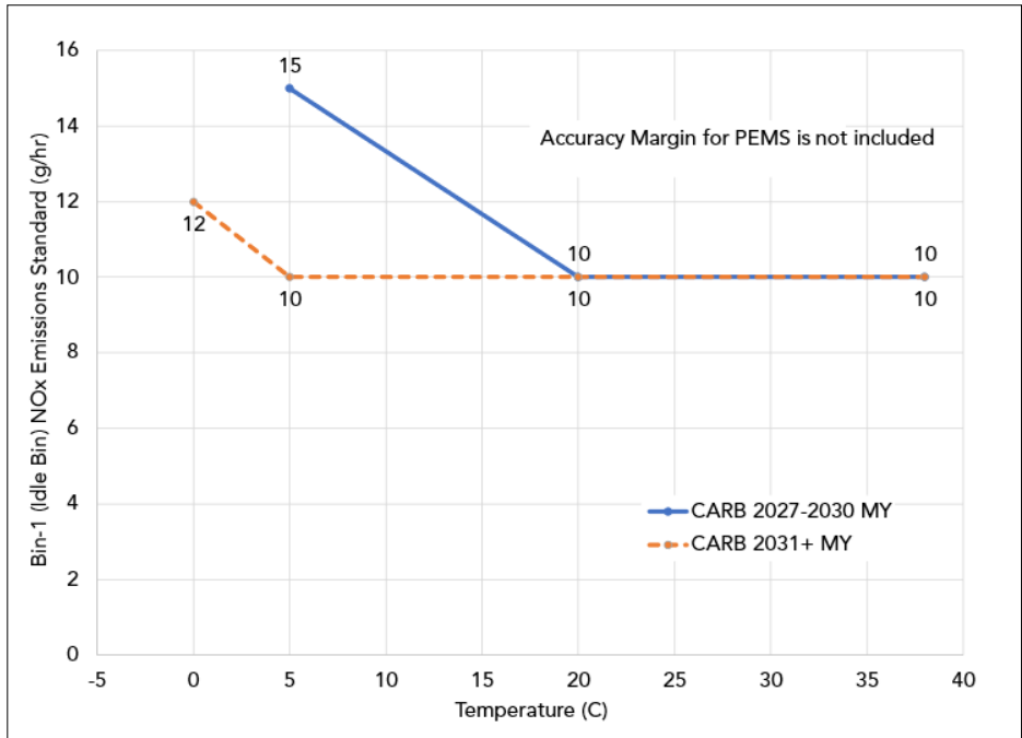
Fig. 3 – CARB Proposal for Bin-1 (Idle Bin) Off-Cycle NOx 1 Emissions Standards. Applicable to LHDD, MHDD, HHDD Engines
