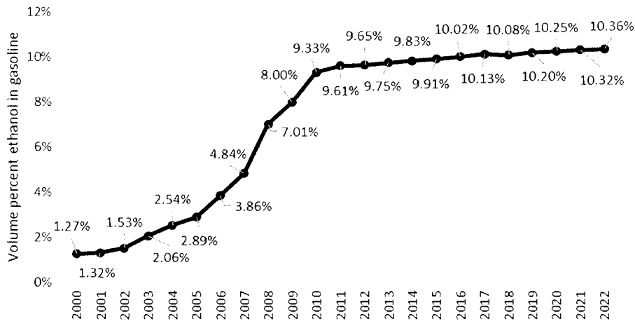
Figure III.B.5-1: Poolwide Ethanol Concentration Over Time
