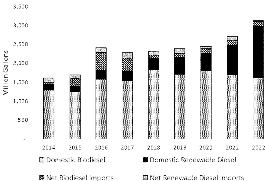
Figure III.B.2-1: Biodiesel and Renewable Diesel Supply 2014–2022 a
