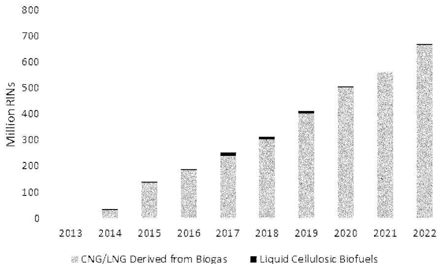
Figure III.B.1-1: Cellulosic Biofuel RINs Generated (2013–2022)
