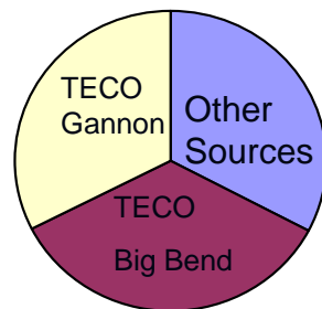
Pre-Clean Up NOx Inventory for Tampa Bay
